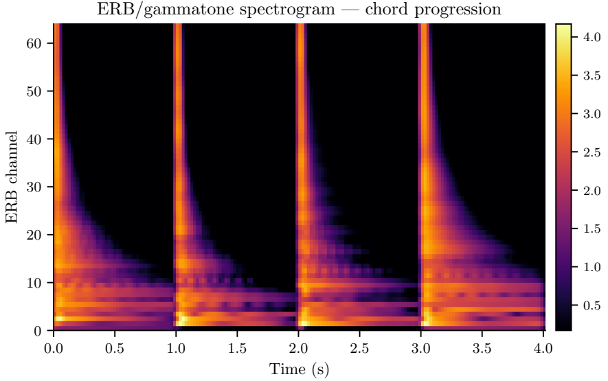
Figure 16: ERB/gammatone spectrogram of the chord progression (log-power scale, 64 channels from 80 Hz to 8 kHz). Each channel’s bandwidth grows with frequency following the ERB function, providing finer frequency resolution in the low-frequency region where harmonic relationships are most salient.
