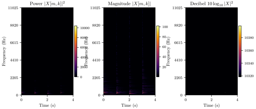
Figure 7: Three amplitude representations of the same spectrogram (Hanning window, N=2048 , 50% hop, f_s=22,050 Hz) computed from a four-chord piano progression. Left: power |X[m, k]|^2 —extremely wide dynamic range makes quiet components invisible. Centre: magnitude |X[m, k]| —square-root compression reveals more structure. Right: decibel scale 10 \log_{10} |X|^2 —perceptually linear, with the harmonic series of each chord clearly legible. The dB representation is standard for analysis and display.
