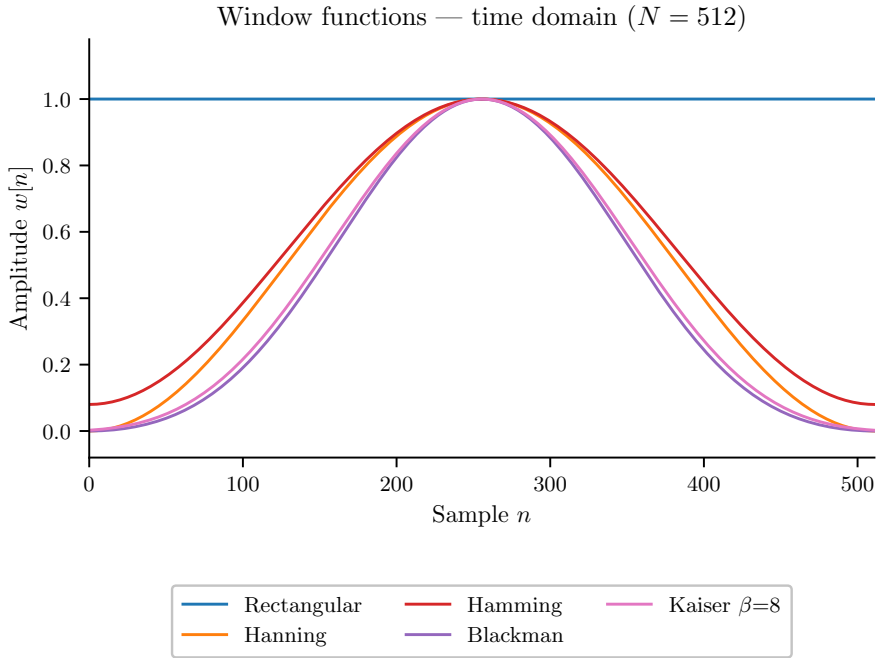
Figure 3: Window functions in the time domain ( N = 512 samples). All windows taper smoothly to reduce discontinuities at the frame boundaries; the rectangular window (uniform weight) is the limiting case with no taper.
