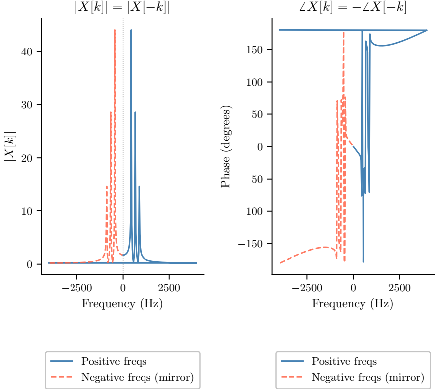
Figure 2: Hermitian symmetry of the full DFT for a real-valued chord signal ( N = 256 , f_s = 8 kHz). Left: magnitude |X[k]| is symmetric about DC—the negative-frequency half is a mirror of the positive-frequency half. Right: phase \angle X[k] is antisymmetric. Only the N/2 + 1 unique bins (positive frequencies, blue) need to be stored; the red dashed curve is entirely redundant.
