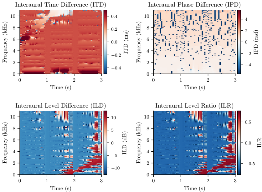
Figure 18: Binaural spectrograms for a simulated two-source scene: a piano chord at 30^\circ right ( \text{ITD} \approx 340 \mu\text{s} , \text{ILD} \approx 8 \text{ dB} ) mixed with a chirp at 60^\circ left. All four cues are shown as time-frequency maps (red = rightward/positive, blue = leftward/negative). ITD is most reliable at low frequencies ( < 1.5 \text{ kHz} ); IPD wraps at high frequencies due to sub-wavelength ambiguity; ILD dominates above 1.5 \text{ kHz} where the head creates an acoustic shadow; ILR normalises the power asymmetry to [-1, +1] and is interpretable at all frequencies.
