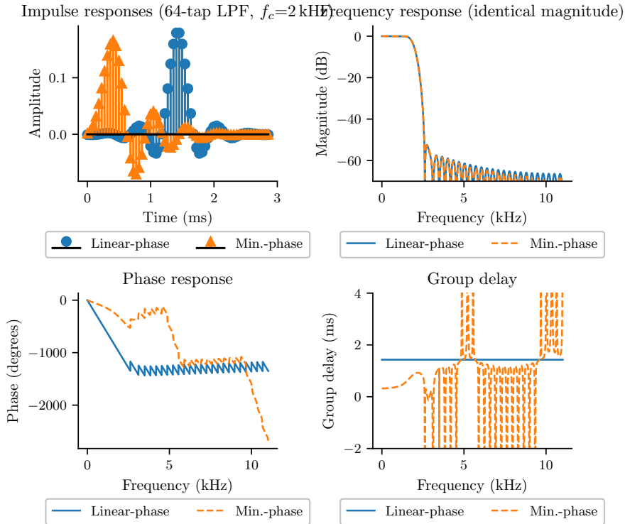
Figure 20: Linear-phase vs. minimum-phase conversion of a 64-tap low-pass FIR filter ( f_c = 2 kHz, f_s = 22050 Hz, Hamming window) via the real-cepstrum method. Top-left: impulse responses—the linear-phase filter (blue) is symmetric around its centre tap; the minimum-phase equivalent (orange) concentrates energy at the start. Top-right: magnitude responses—both filters share identical frequency responses; only the phase differs. Bottom-left: phase responses. Bottom-right: group delay—the linear-phase filter introduces (L - 1)/2 \approx 1.45 ms of constant latency; the minimum-phase design reduces this to near zero, enabling low-latency room correction and live processing.
