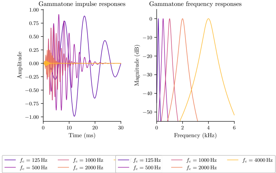
Figure 12: Gammatone auditory filters at five centre frequencies (125 Hz, 500 Hz, 1 kHz, 2 kHz, 4 kHz). Left: time-domain impulse responses (order n=4 , bandwidth b=1.019 \cdot \text{ERB}(f_c) ). The envelope t^{n-1}e^{-2\pi b t} shortens at higher frequencies because the ERB bandwidth grows with f_c . Right: frequency responses showing the characteristic asymmetric skirt of the auditory filter—sharper on the high-frequency side, broader toward lower frequencies.
