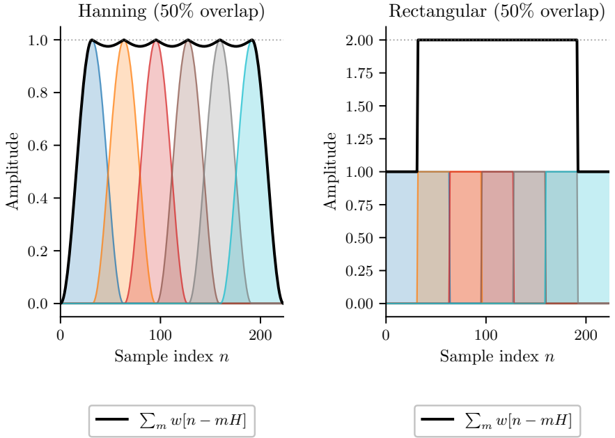
Figure 6: Constant Overlap-Add (COLA) visualisation for six overlapping frames ( N = 64 , 50% hop). Left: Hanning window—the coloured envelopes sum (black curve) to a constant, guaranteeing perfect reconstruction. Right: rectangular window—also constant, confirming that any non-zero hop satisfies COLA for the rectangular case.
