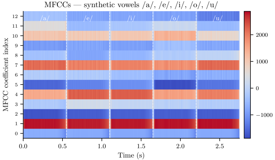
Figure 14: MFCCs ( C=13 ) computed from five synthesised vowels (/a/, /e/, /i/, /o/, /u/, each \approx 0.55 s). Vertical white dashes mark vowel transitions. The low-order coefficients (rows 0–4) encode the broad spectral envelope (vowel identity), while higher-order coefficients capture finer spectral detail. The DCT-II decorrelates the mel-band energies, concentrating the discriminative information into the first few coefficients—which is why 13 MFCCs are sufficient for most speech tasks.
